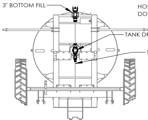
BOTTOM VIEW - CONE BOTTOM TANK
