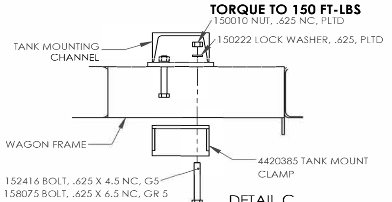
DETAIL C SCALE 1 : 10
