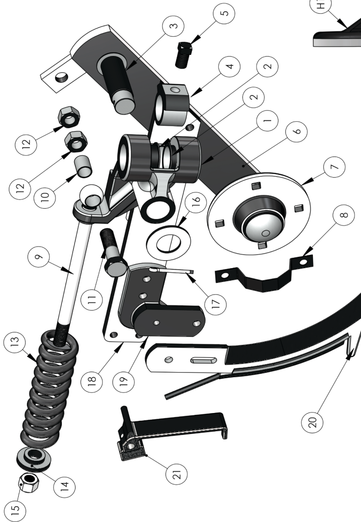
B.O.M FOR COULTER HUB ASSEMBLY
